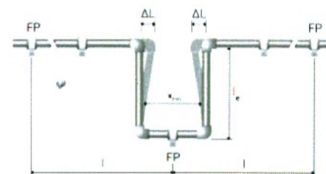
Figure 1—Omega and U part
